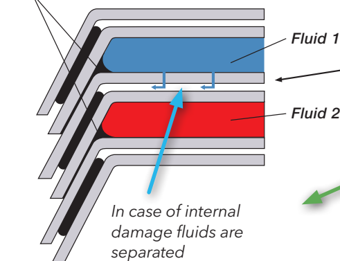
Brazing Material
