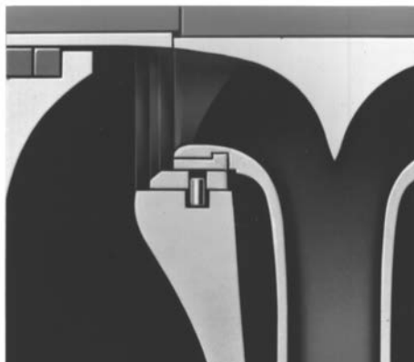
Impeller Wearing Rings
